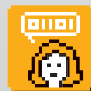
E-skills
