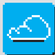
Cloud Computing
