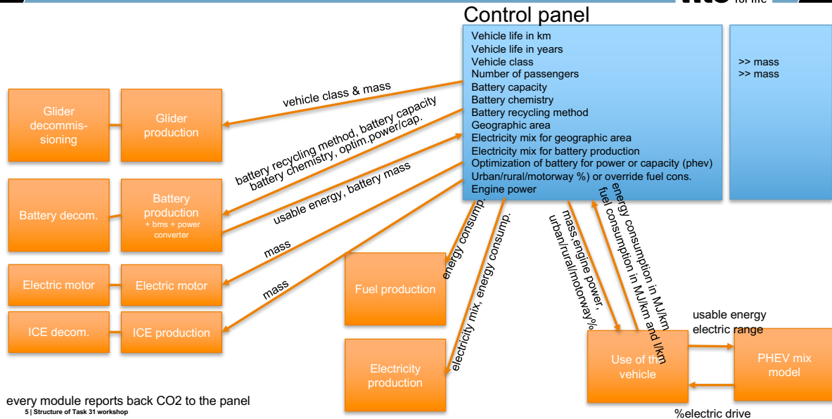
Figure 3 Schematic representation of the T31 model illustrating the different calculation modules and the control panel choices which can be modified by the user
