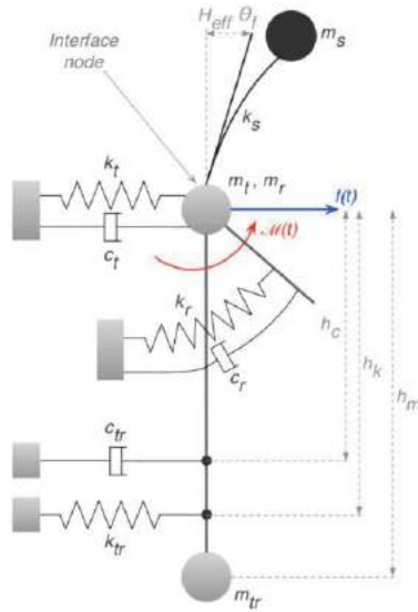
Figure 2.5 The lumped parameter elastic SSI model
