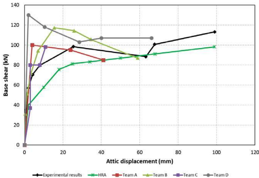
Figure 2.4 Comparing blind-predictions with experimental results for EUC-BUILD6
