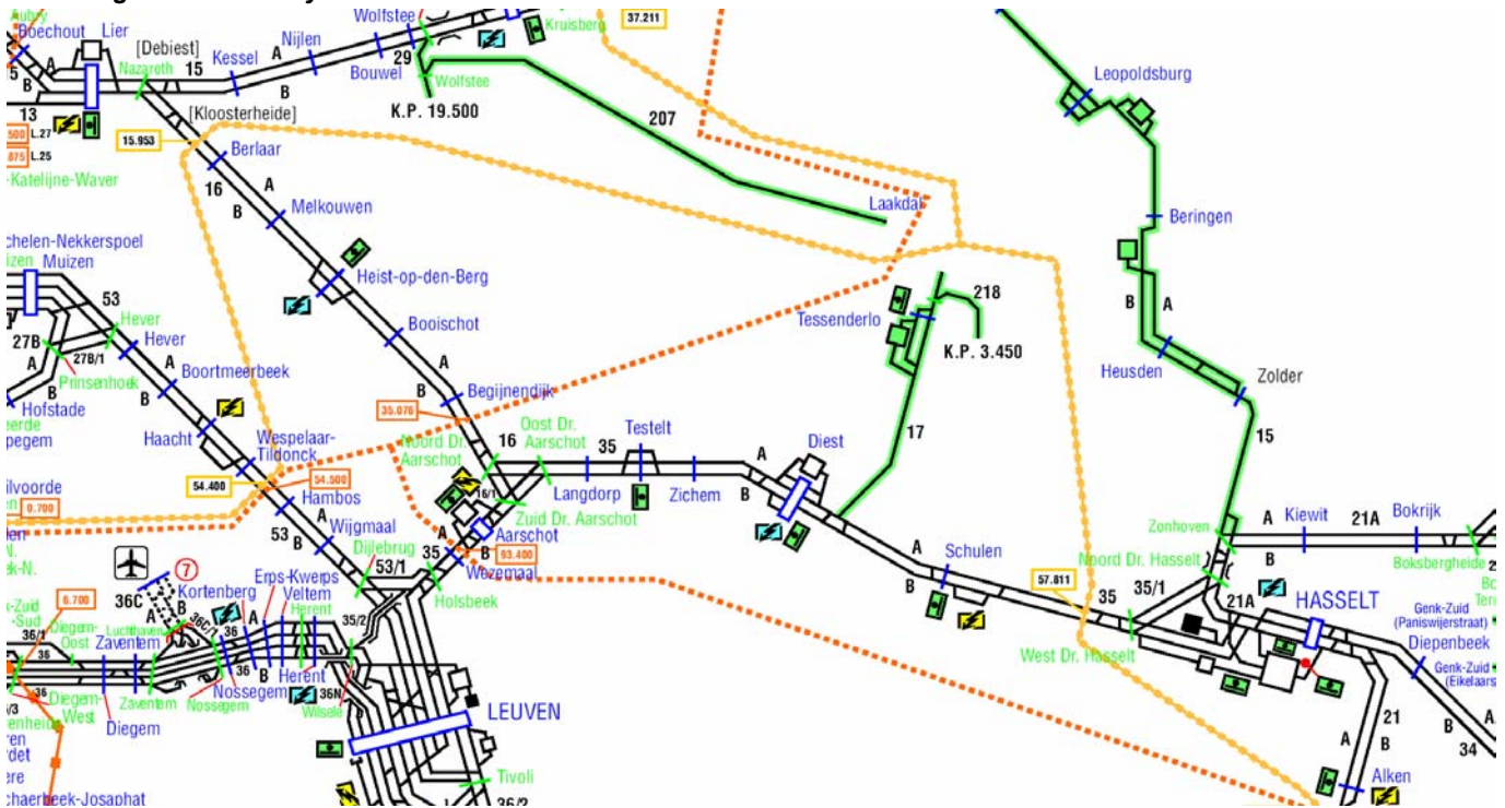
Figure 36: Railway network around Aarschot
