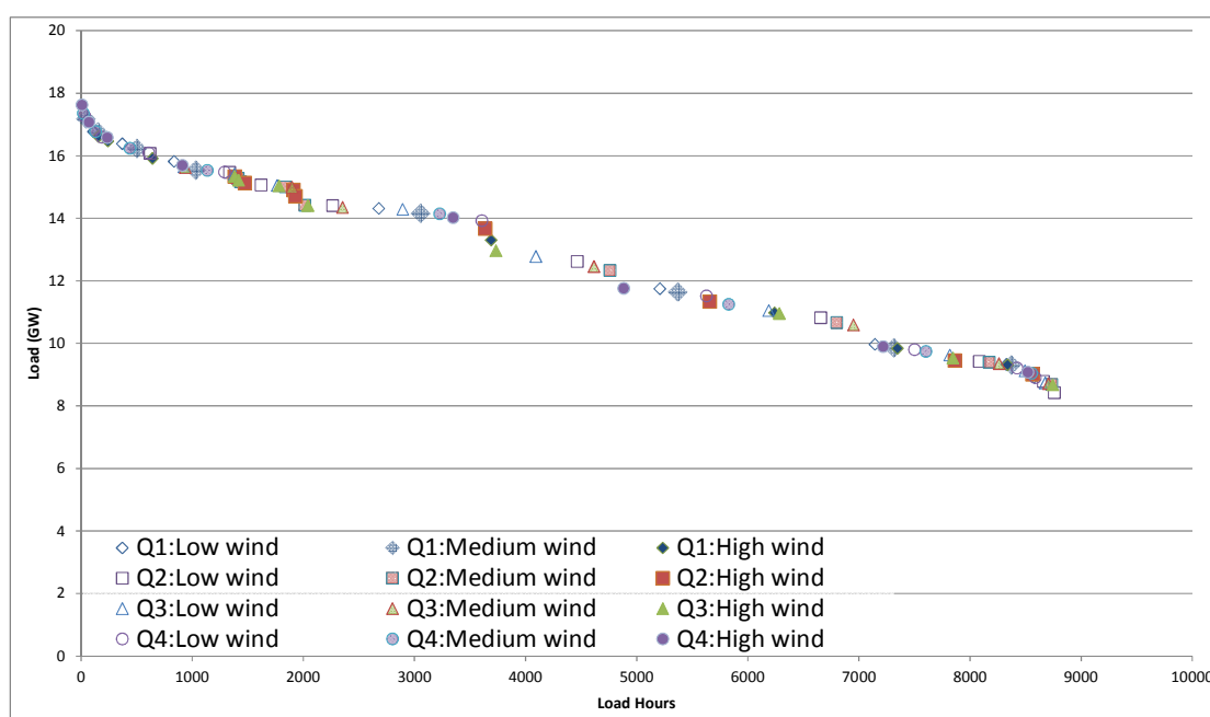
Figure B.5 Selected Bands in Load Duration Curve
