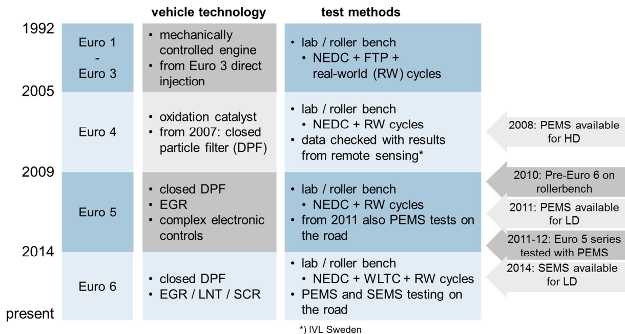
Figure 1 Overview of how the measurement program applied by TNO for testing LD diesel vehicles has evolved together with the evolution of vehicle technology and available test methods
